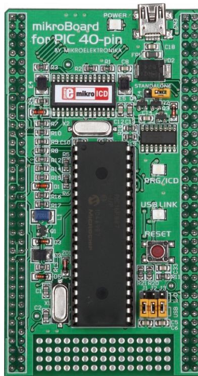
Figure 1: mikroBoard for PIC 40-pin
