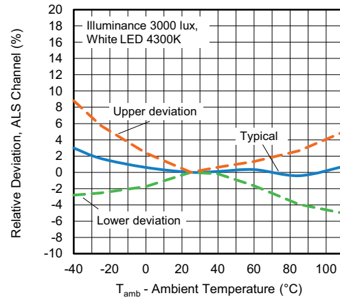
Fig. 8 - Relative Deviation, ALS Channel vs. Temperature (at lux levels lower than ~200 lux, dark current effects should be taken into account)
