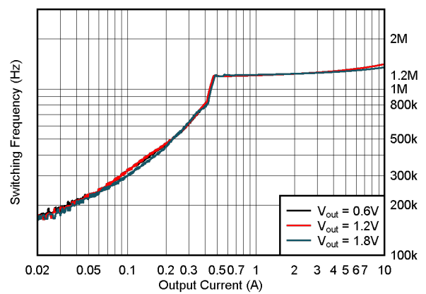
V_{IN} = 3.3V T_A = 25^\circ C PFM Figure 9-14. Switching Frequency
