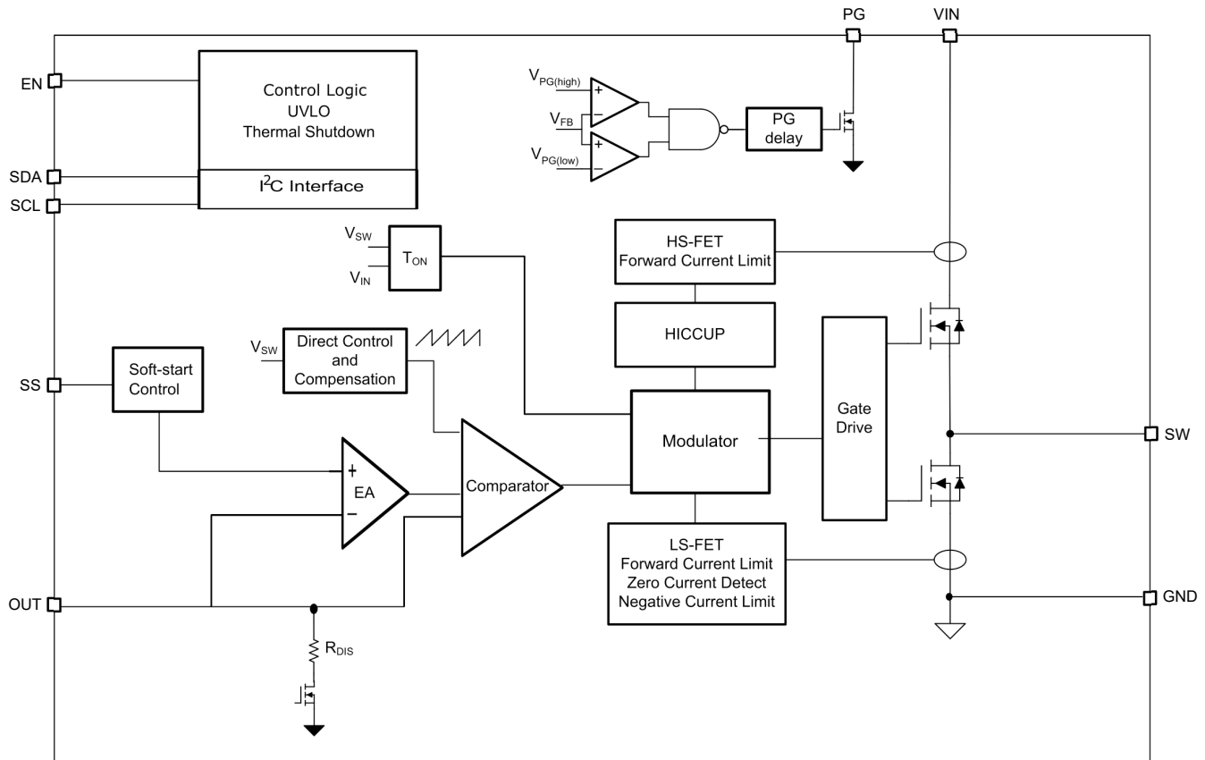
Figure 7-2. Functional Block Diagram - I²C Version (TPS6286Bxx)
