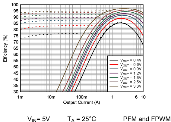
Figure 9-4. Efficiency vs Output Current
