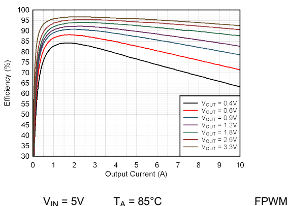
Figure 9-8. Efficiency vs Output Current
