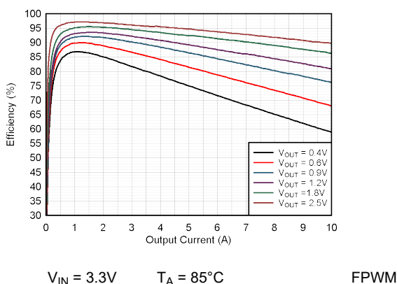
Figure 9-9. Efficiency vs Output Current
