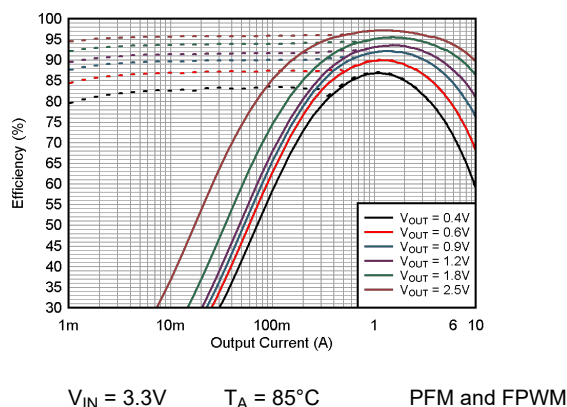
Figure 9-7. Efficiency vs Output Current
