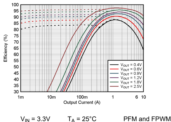
Figure 9-5. Efficiency vs Output Current
