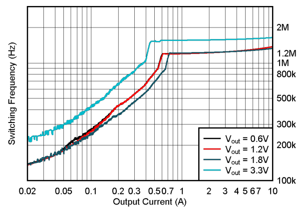
V_{IN} = 5.0V T_A = 25^\circ C PFM Figure 9-15. Switching Frequency
