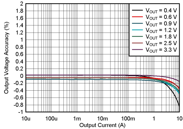
V_{IN} = 5V T_A = 25^\circ C FPWM Figure 9-12. Load Regulation
