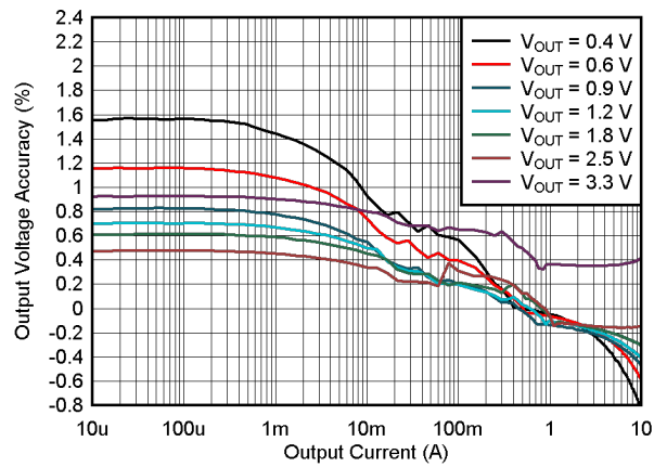
V_{IN} = 5V T_A = 25^\circ C PFM Figure 9-10. Load Regulation
