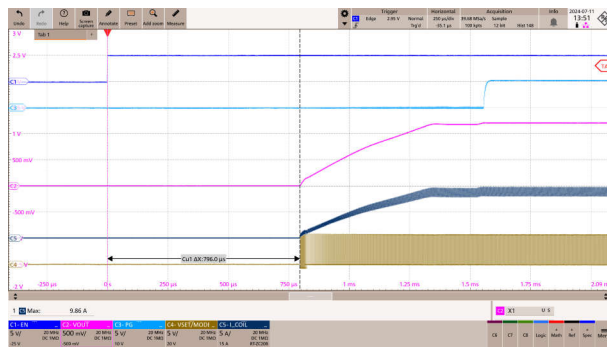
Figure 9-22. FPWM Operation
