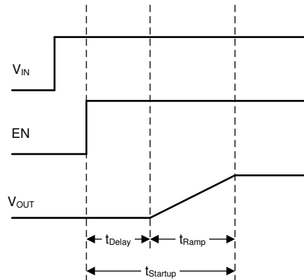
Figure 7-3. Start-Up Sequence
