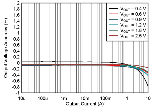
V_{IN} = 3.3V T_A = 25^\circ C FPWM Figure 9-13. Load Regulation
