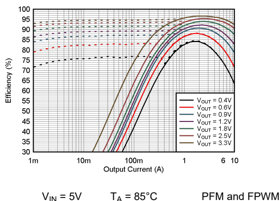
Figure 9-6. Efficiency vs Output Current
