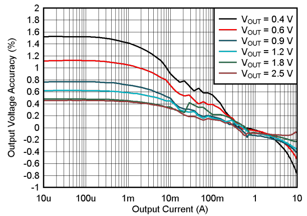
V_{IN} = 3.3V T_A = 25^\circ C PFM Figure 9-11. Load Regulation
