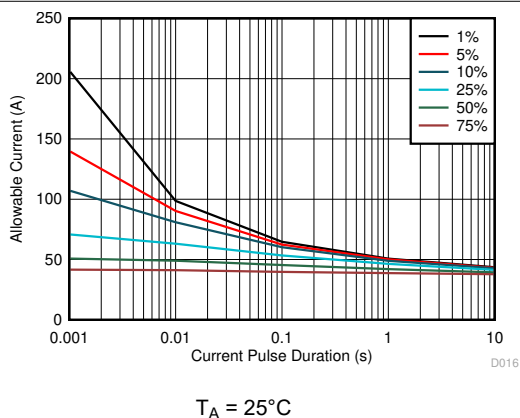
Figure 8-6. Maximum Repetitive Pulsed Current vs Pulse Duration
