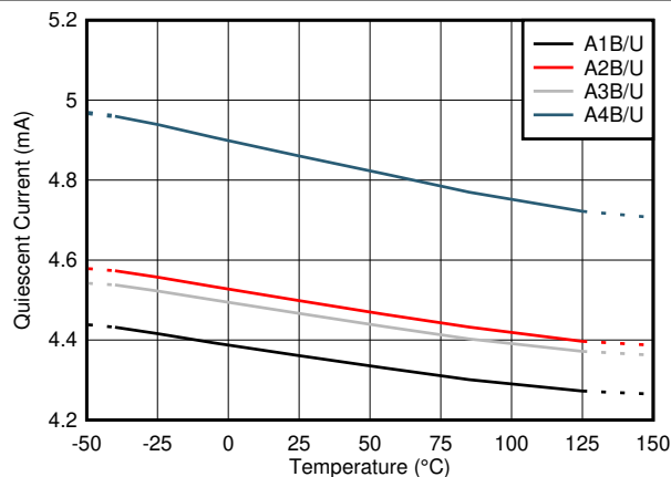
Figure 7-7. Quiescent Current vs Temperature
