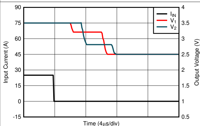
Figure 7-10. Voltage Output Step, Falling
