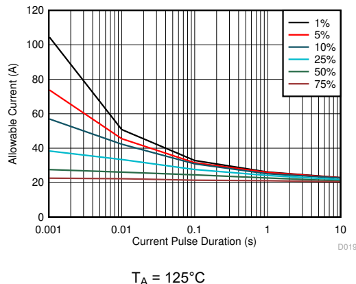
Figure 8-9. Maximum Repetitive Pulsed Current vs Pulse Duration
