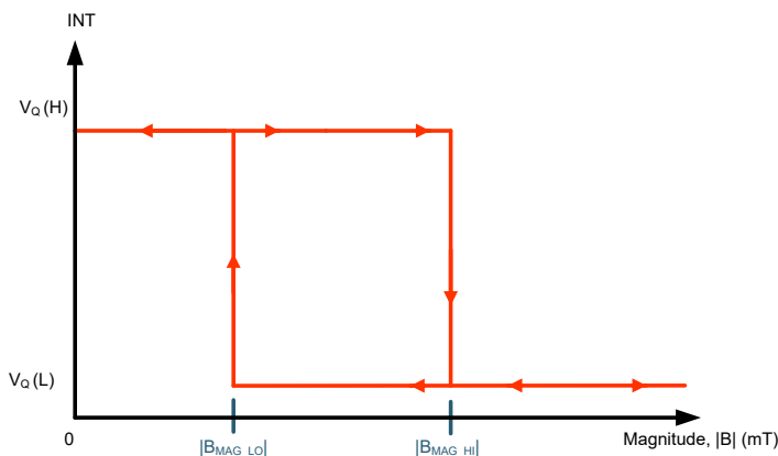
Figure 8-17. Magnitude Switch
