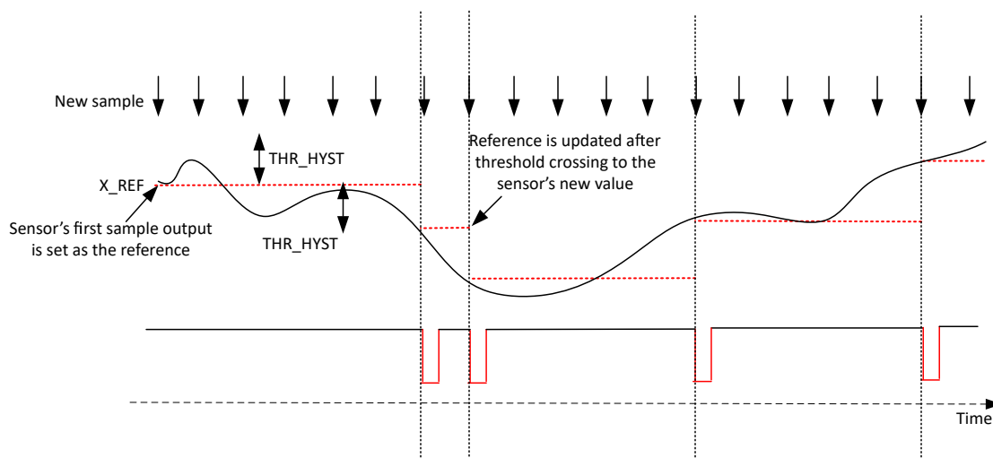
Figure 6-8. Wake on Change With Magnetic Axes Measurements , WOC_SEL = 2h, INT_State = 1h
