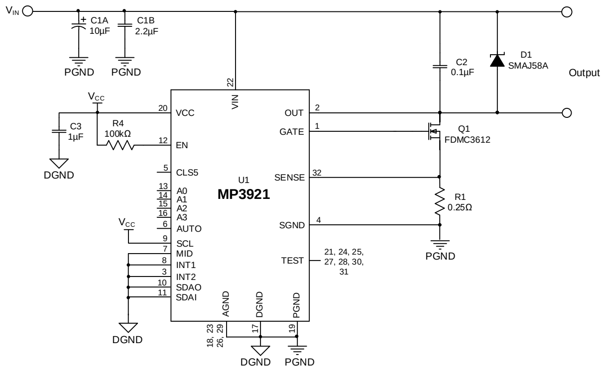
Figure 18: Typical Application Circuit (without I 2 C Control)
