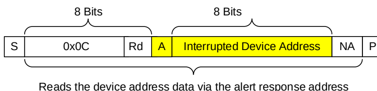
Figure 14: I 2 C Read Example
