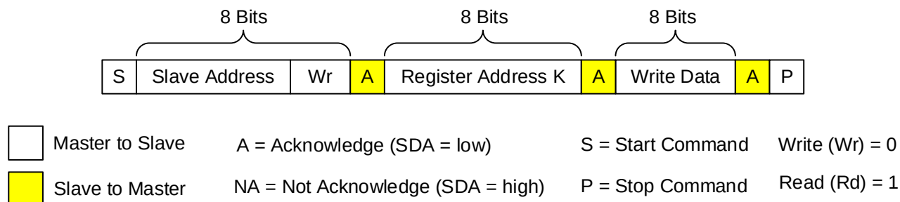
Figure 13: I 2 C Write Example
