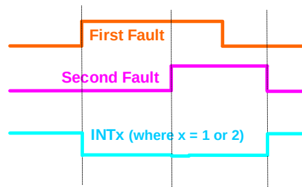
Figure 8: Interrupt Sequence
