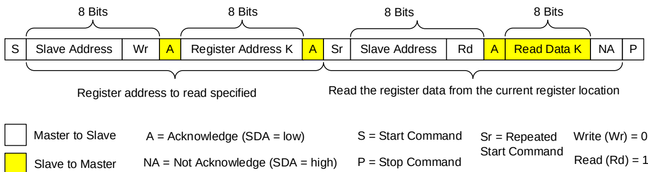
Figure 14: I 2 C Read Example
