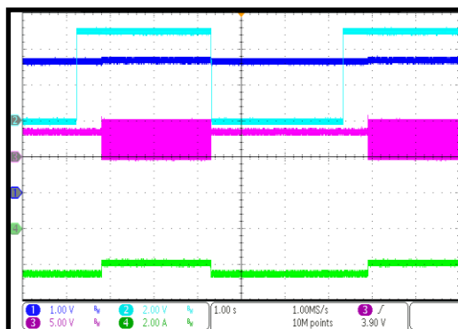
Power-On/Off Waveform
