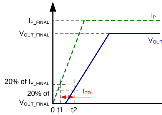
Figure 5: Propagation Delay ( t_{PD} )
