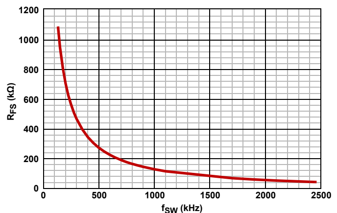
FIGURE 26. R_{FS} vs FREQUENCY
