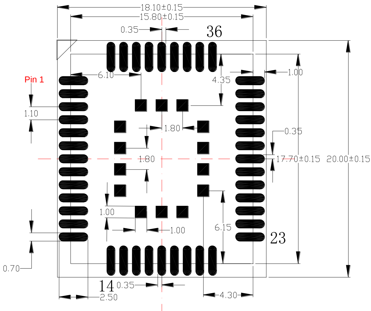
Figure 33: Recommended Footprint (Top View, Unit: mm)
