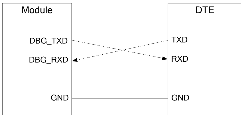
Figure 15: Reference Design for Debug UART Interface
