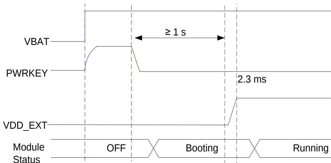
Figure 8: Turn-on Timing
