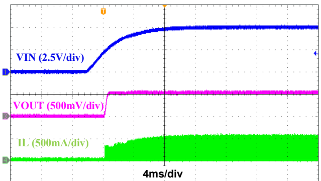
Figure 20. Startup Using V_{IN} , I_{OUT} = 0.1\text{A}
