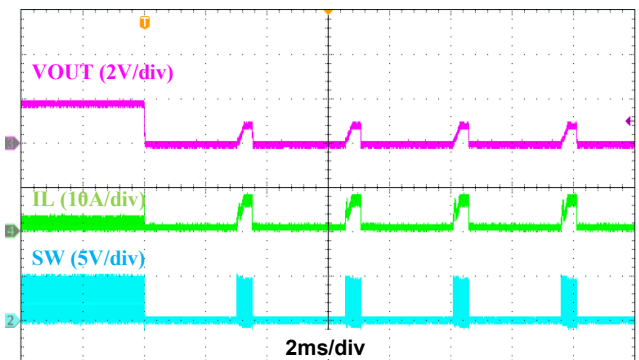
Figure 22. Output Short Protection, I_{OUT} = 0.05\text{A}
