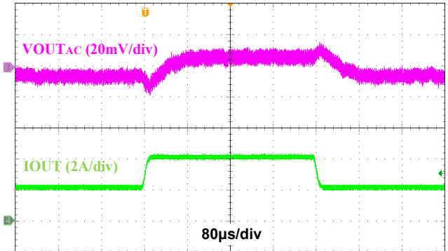
Figure 18. Load Transient, I_{OUT} = 2\text{A} to 4\text{A} to 2\text{A}
