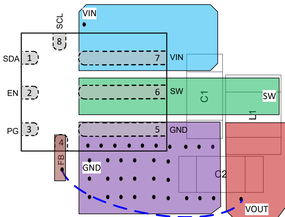
Figure 44. Recommended Layout
