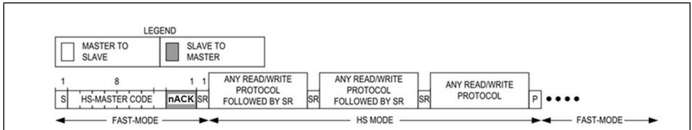
Figure 43. Engaging HS Mode
