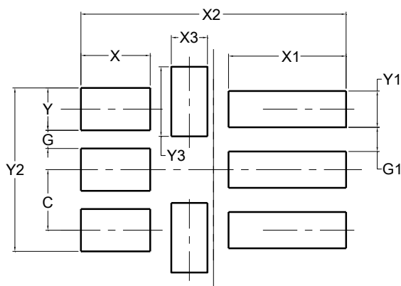
W-QFN1520-8/SWP (Type UX)
