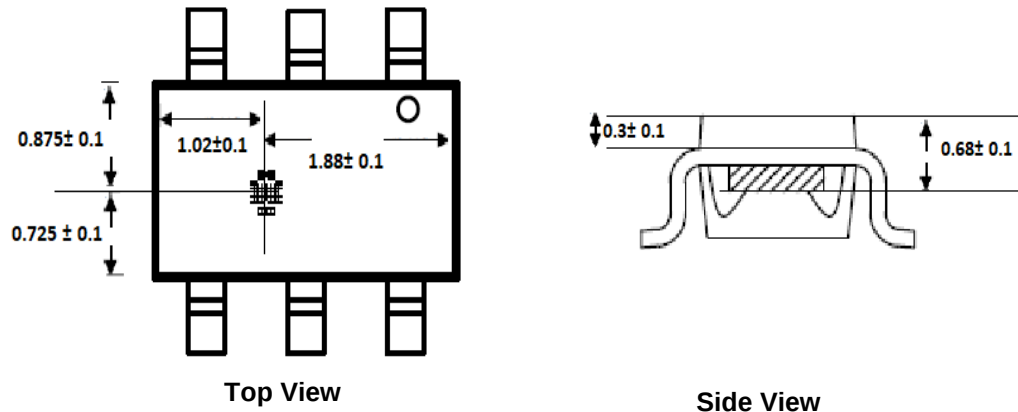
Sensor Location (Unit: mm)
