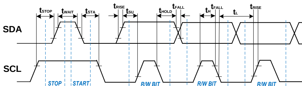
Figure 1. I2C Timing Parameters
