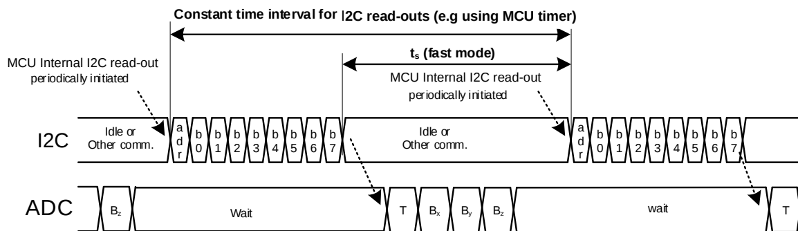
Figure 11. Synchronous, Fast I2C Access Using a Periodic I2C Read-Out
