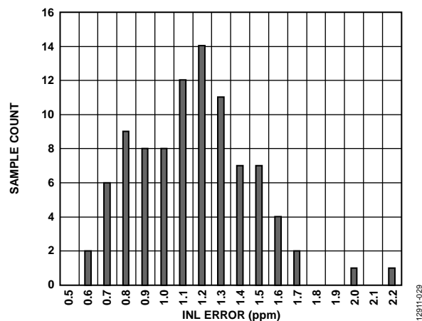
Figure 26. Integral Nonlinearity (INL) Distribution Histogram (All Input Buffers Disabled, Differential Input, V_{REF} = 5 V External, 92 Units)
