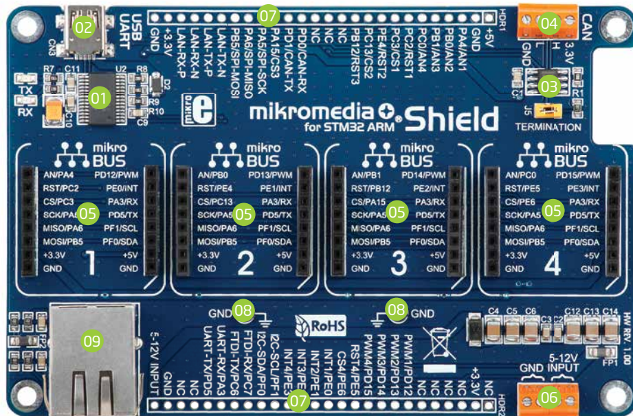
Figure 1-1: mikromedia+ shield
