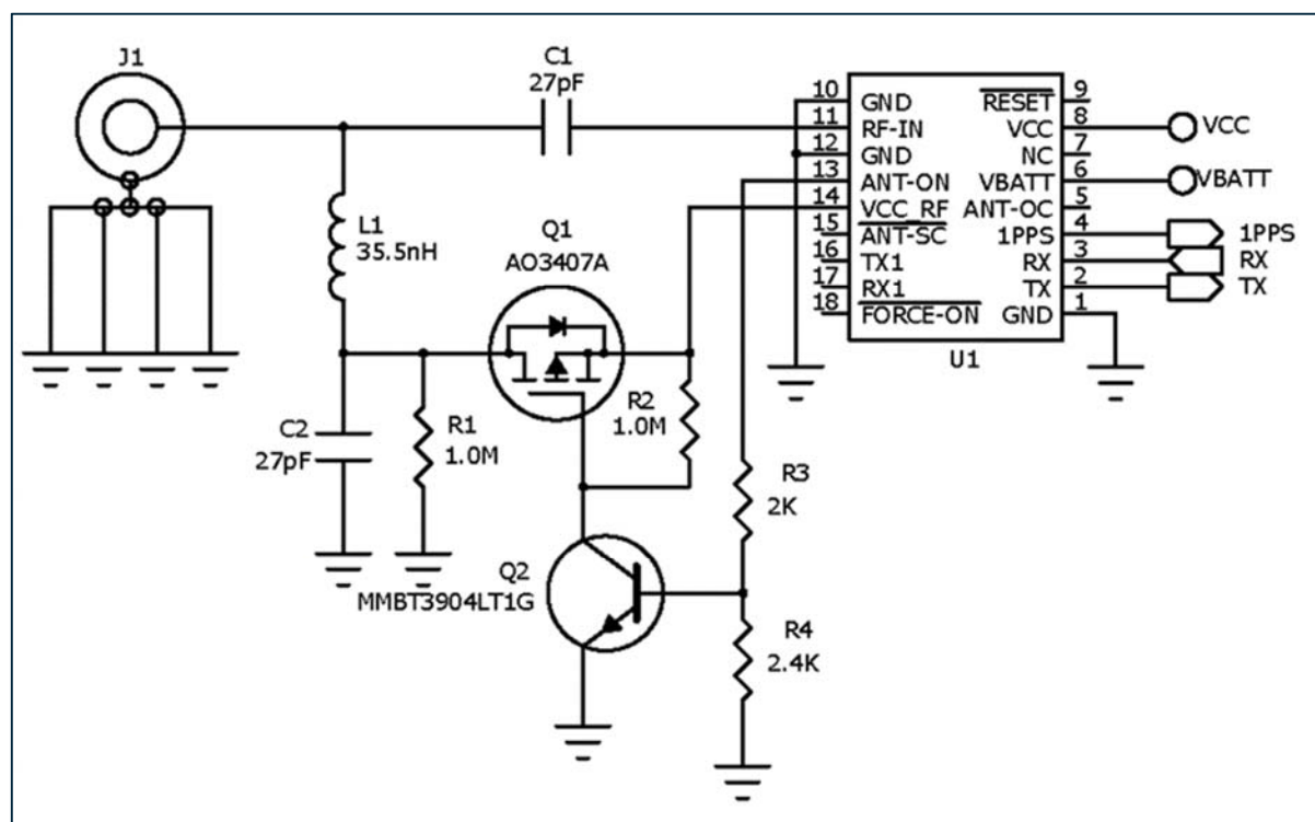
Figure 11-1 SL871 Family Reference Design
