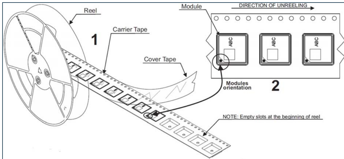
Figure 14-2 Tape and Reel Packaging
