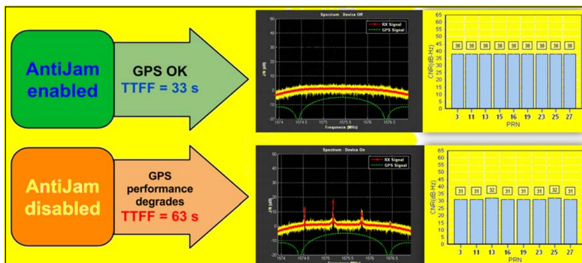
Figure 4-1 Jamming Rejection
