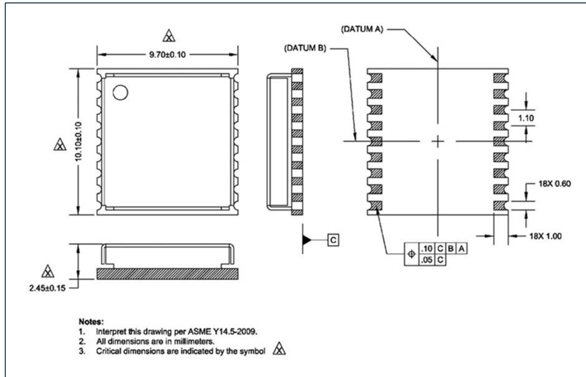
Figure 12-1 SL871 Family Mechanical Drawing
