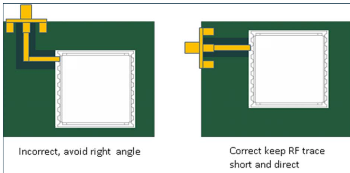
Figure 10-1 RF Trace Examples
