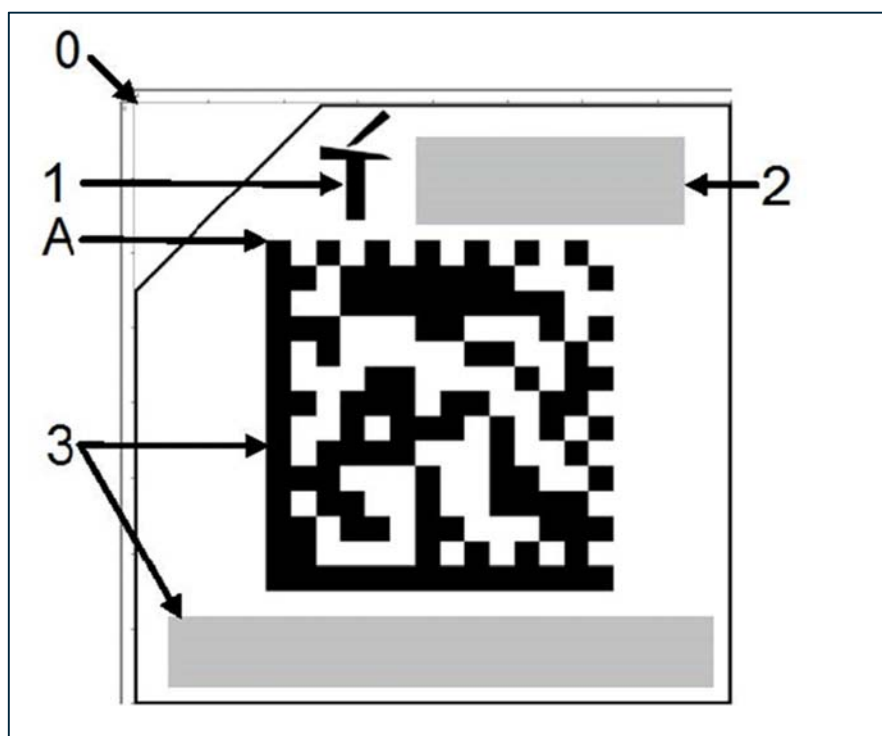
Figure 14-1 Product Label
