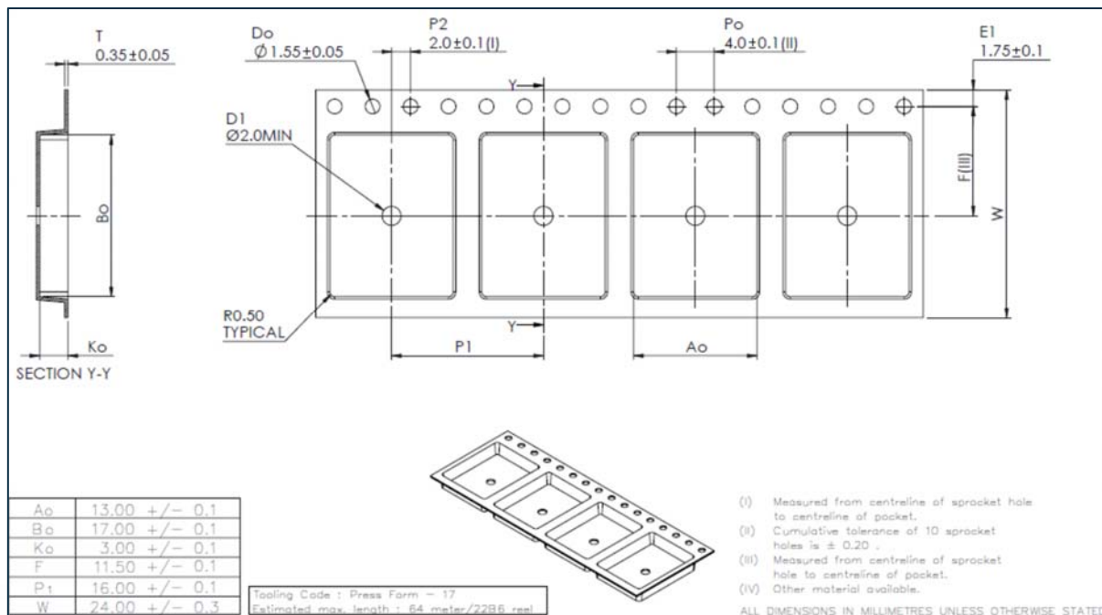
Figure 14-3 Tape and Reel Detail
