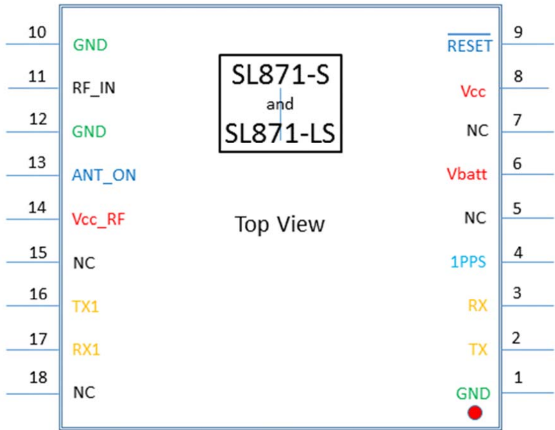
Figure 9-2 SL871-S and SL871L-S Pin-out diagram
