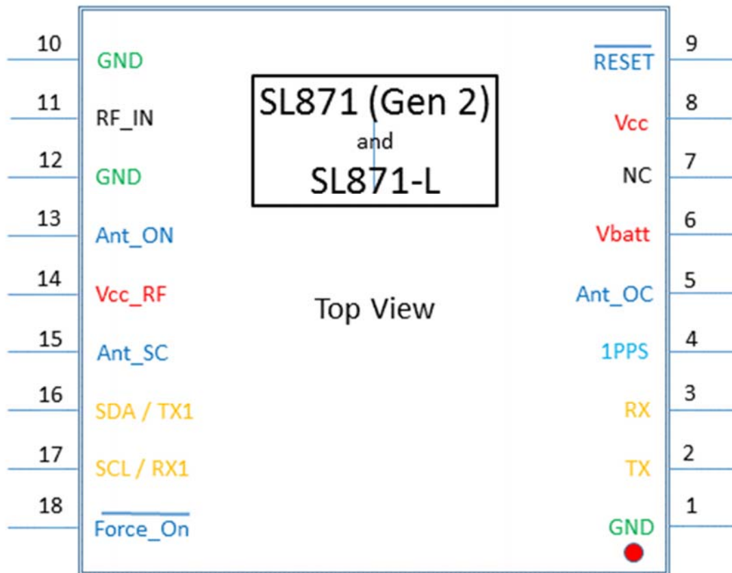
Figure 9-1 SL871 (Gen 2) and SL871L Pin-out diagram
