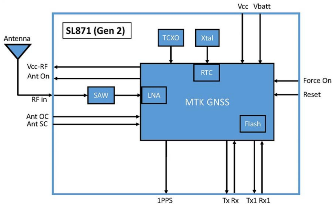
Figure 2-1 SL871 (Gen 2) Block Diagram
