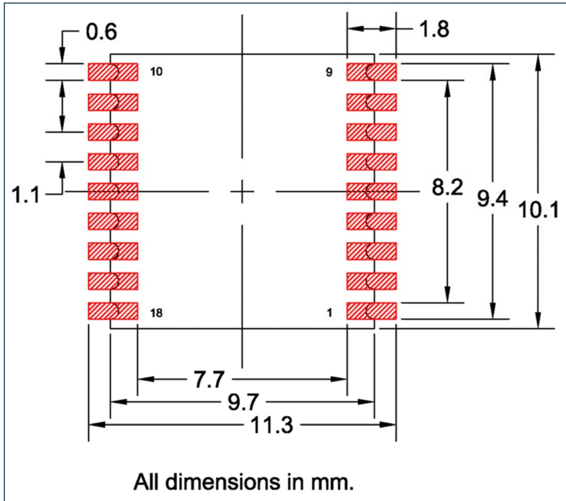
Figure 13-1 SL871 Family PCB Footprint
